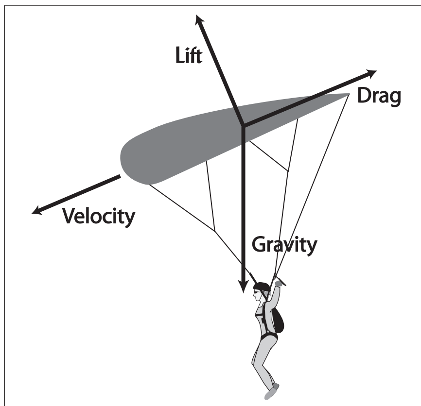
Figure 6-1. The forces acting upon a canopy in flight.
